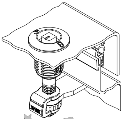
First 90° rotation: the cam latches behind the frame into the locked position. The door cannot be opened.
